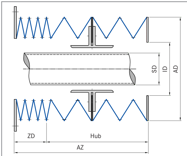
Sectional view HF bellow
